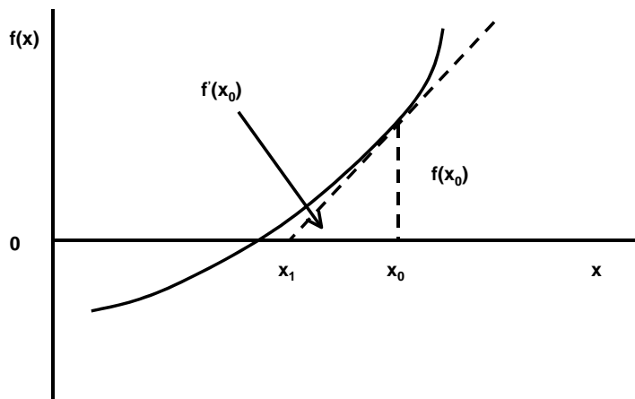
Figure 4: Newton's Method
